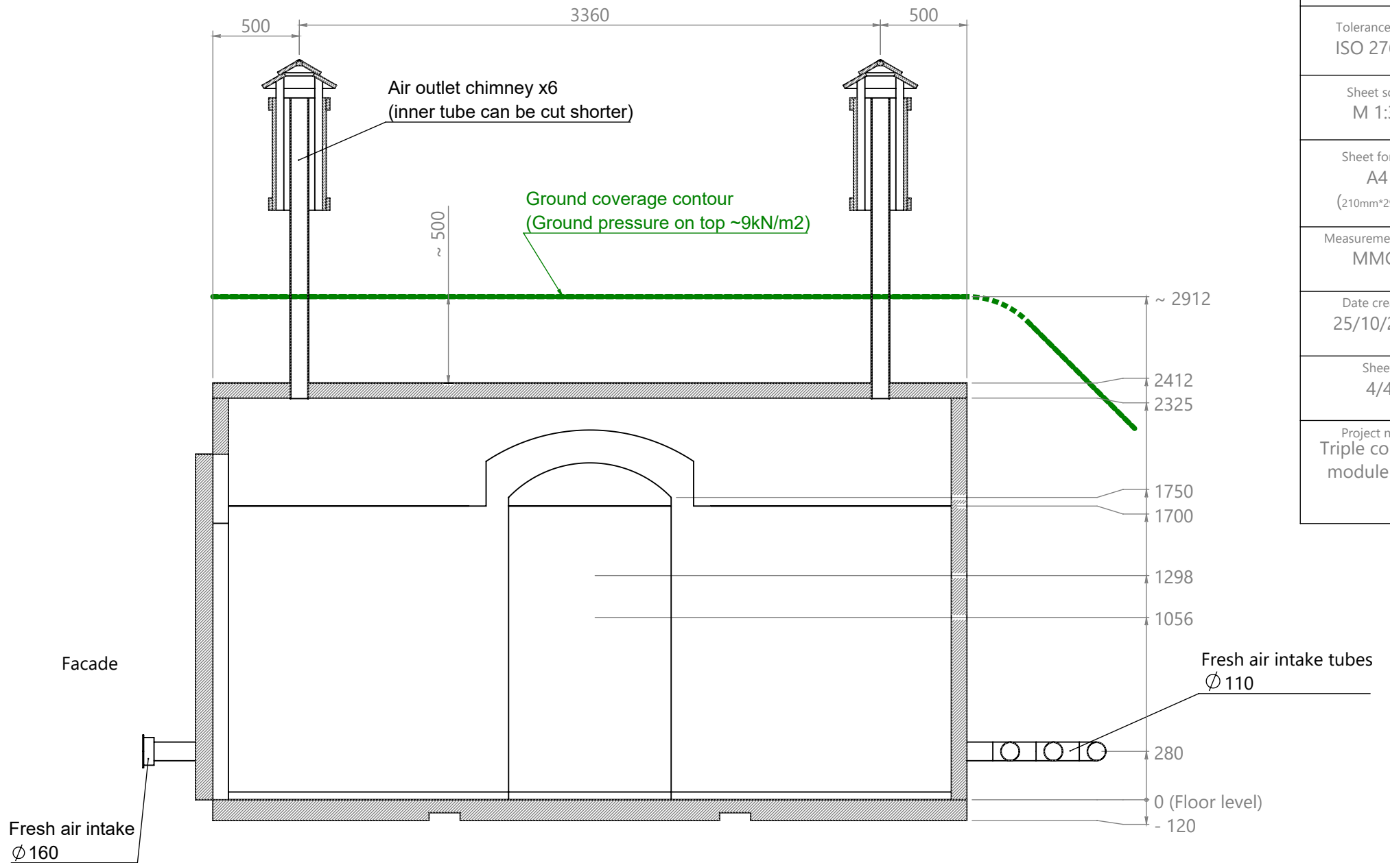
Side section view B-B Dimensions for concrete modules
